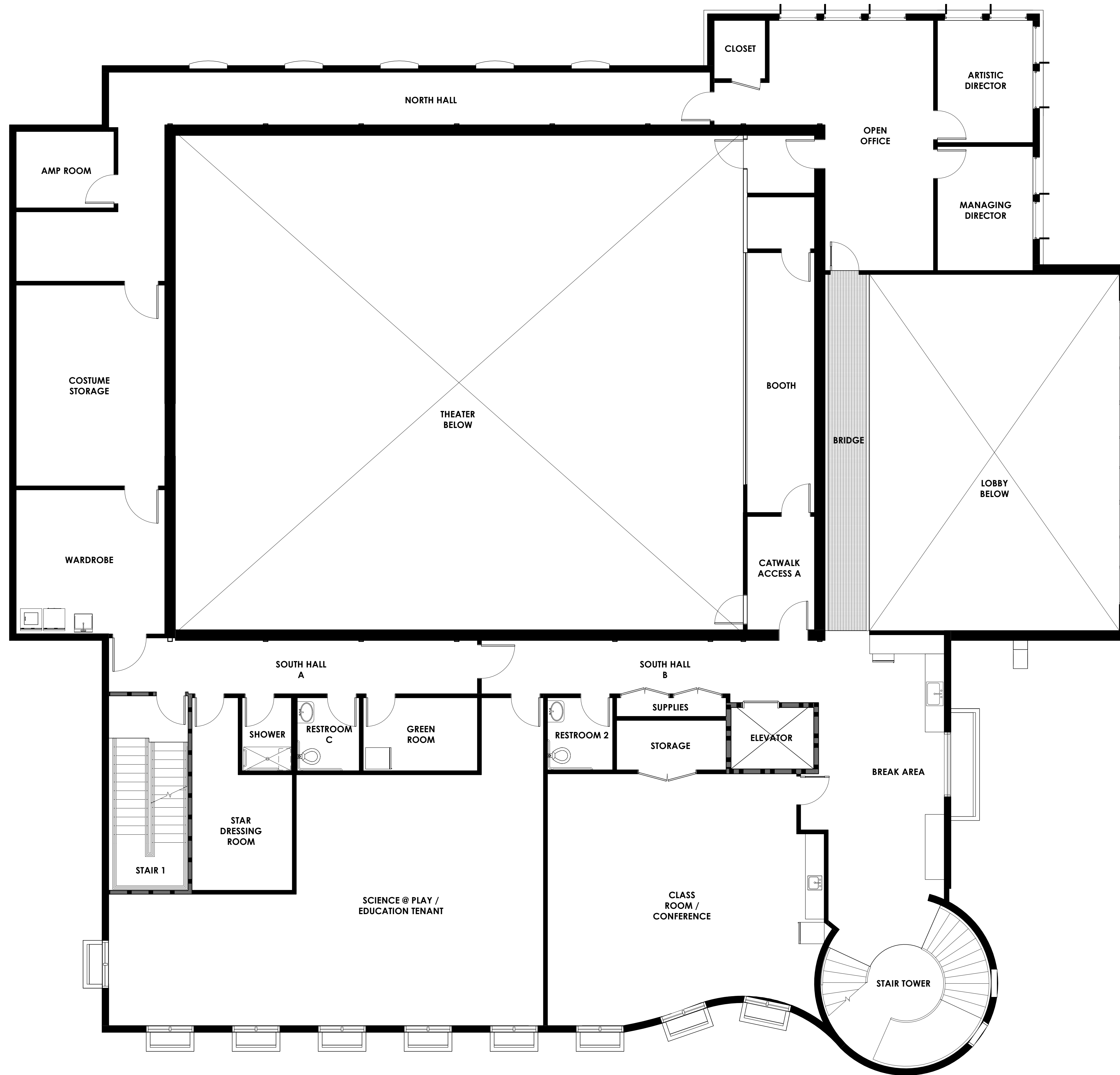
FLOOR 2
